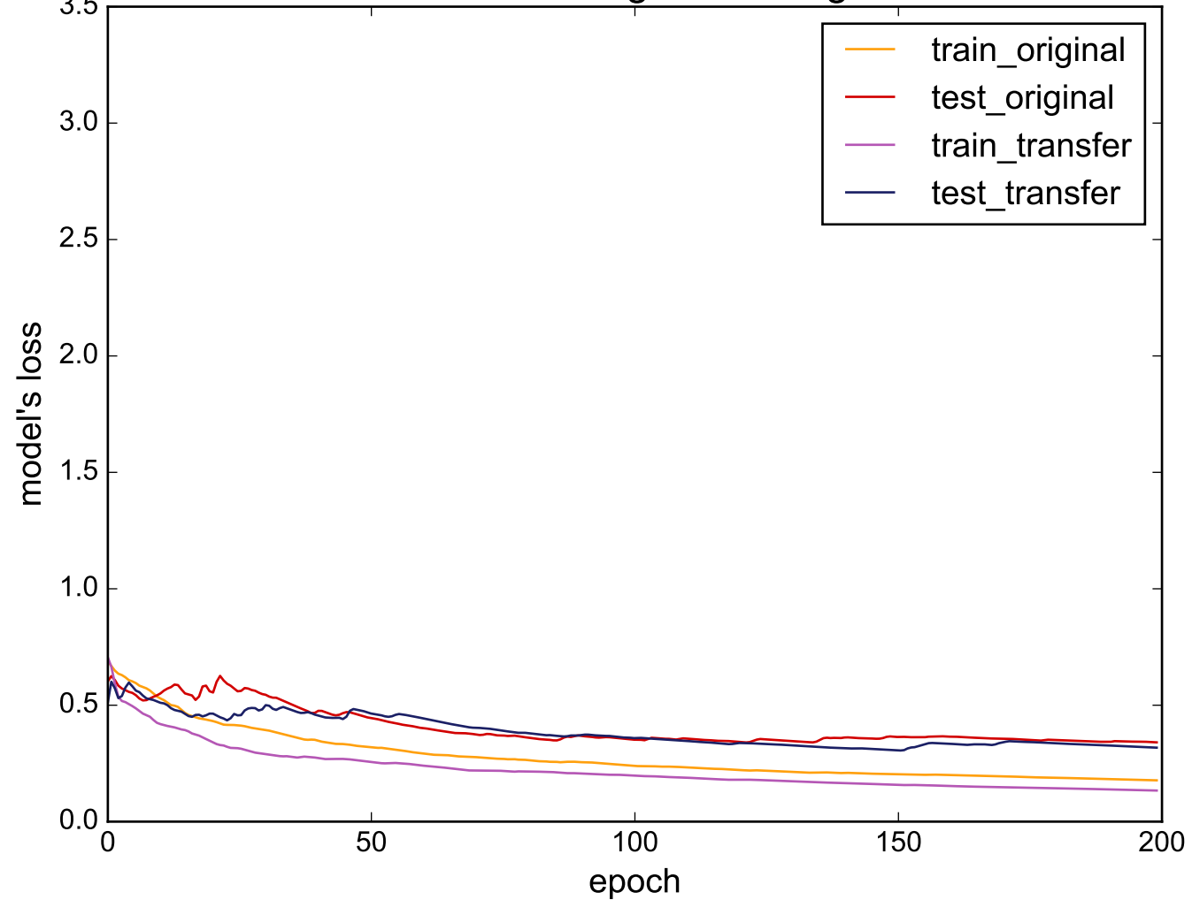
Source: ECG200 - Target: ToeSegmentation1
