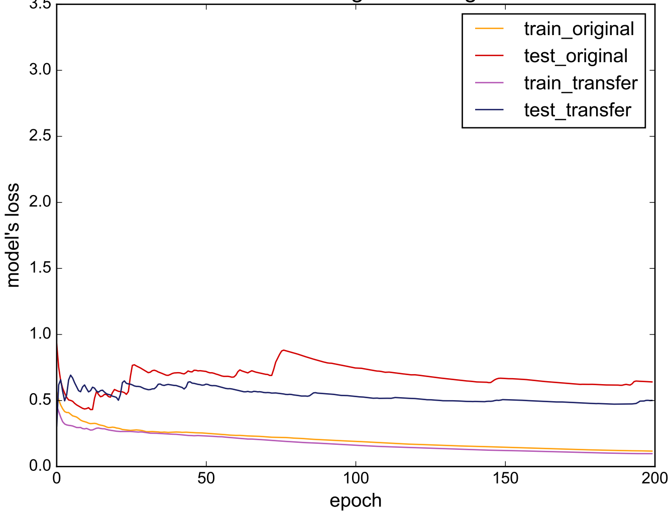
Source: ECG200 - Target: ToeSegmentation2
