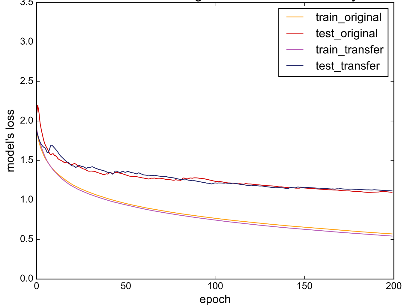
Source: ECG200 - Target: UWaveGestureLibraryAll
