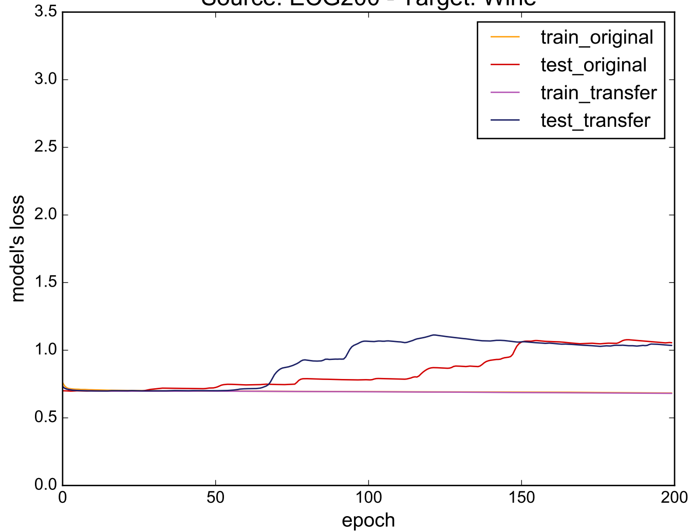
Source: ECG200 - Target: Wine
