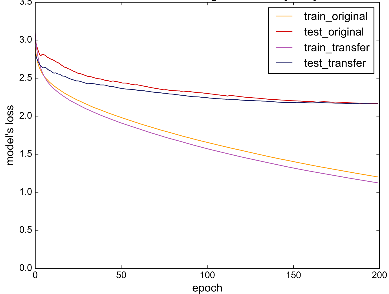
Source: ECG200 - Target: WordsSynonyms
