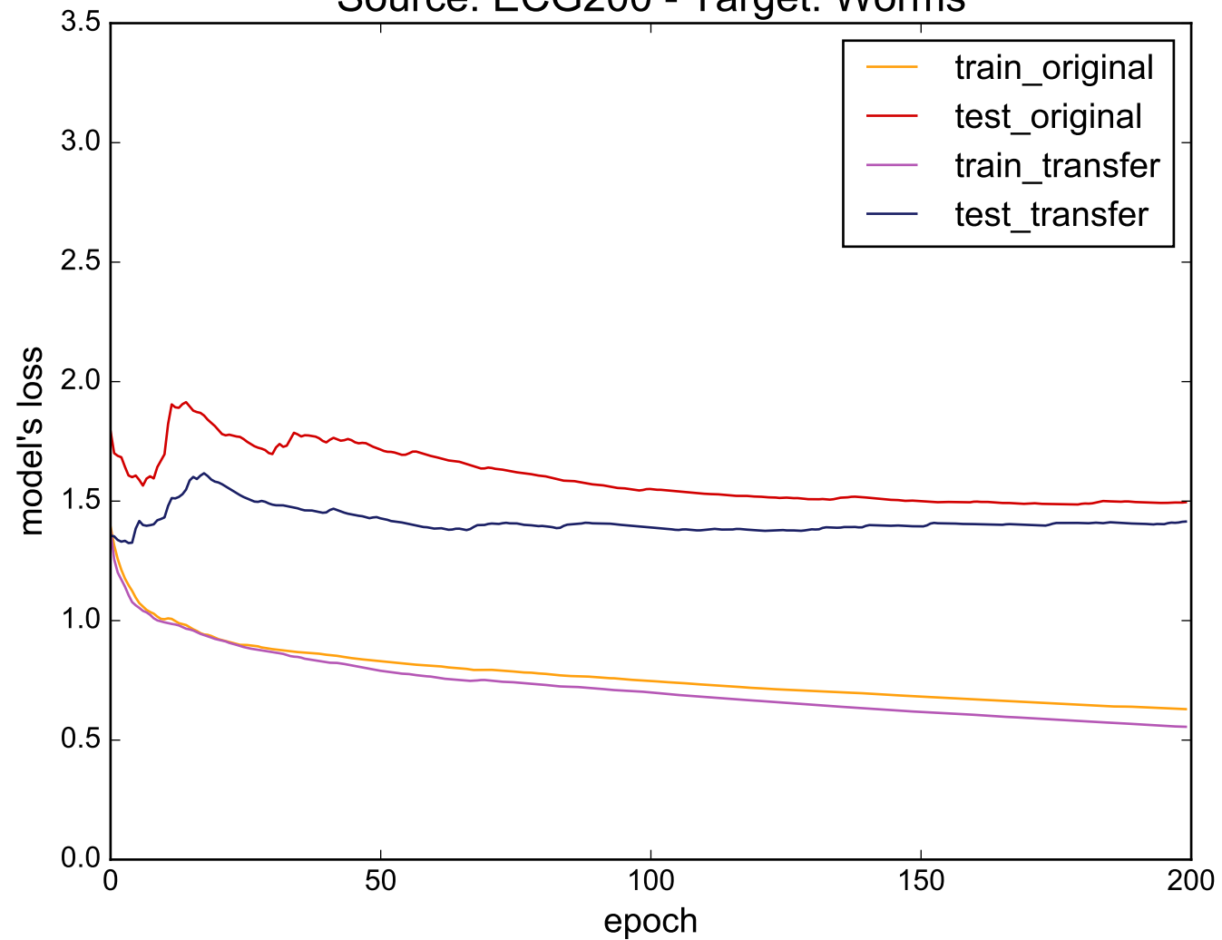
Source: ECG200 - Target: Worms
