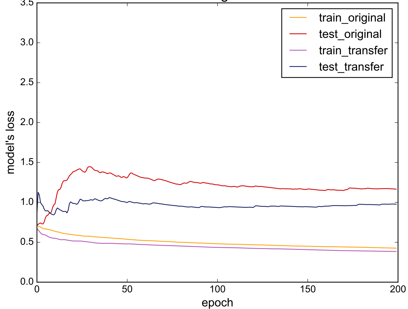
Source: ECG200 - Target: WormsTwoClass
