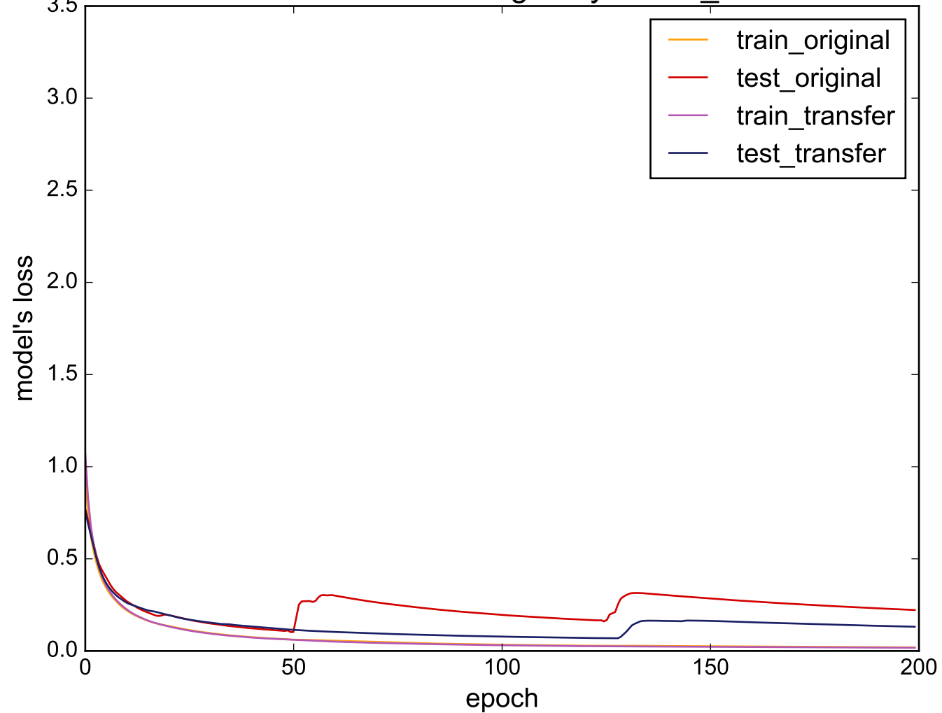
Source: ECG200 - Target: synthetic_control
