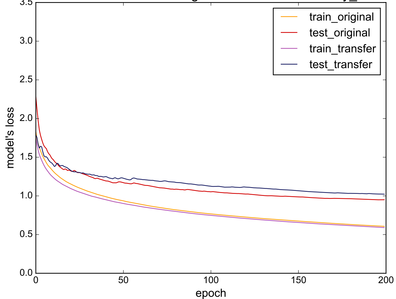
Source: ECG200 - Target: uWaveGestureLibrary_X
