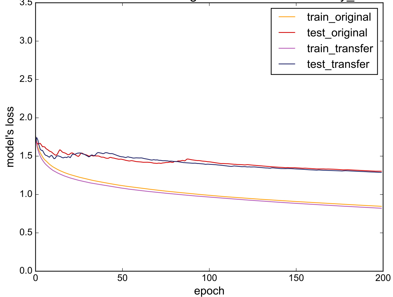
Source: ECG200 - Target: uWaveGestureLibrary_Y
