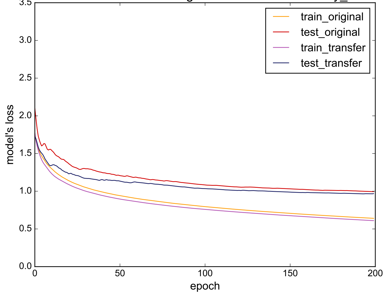
Source: ECG200 - Target: uWaveGestureLibrary_Z
