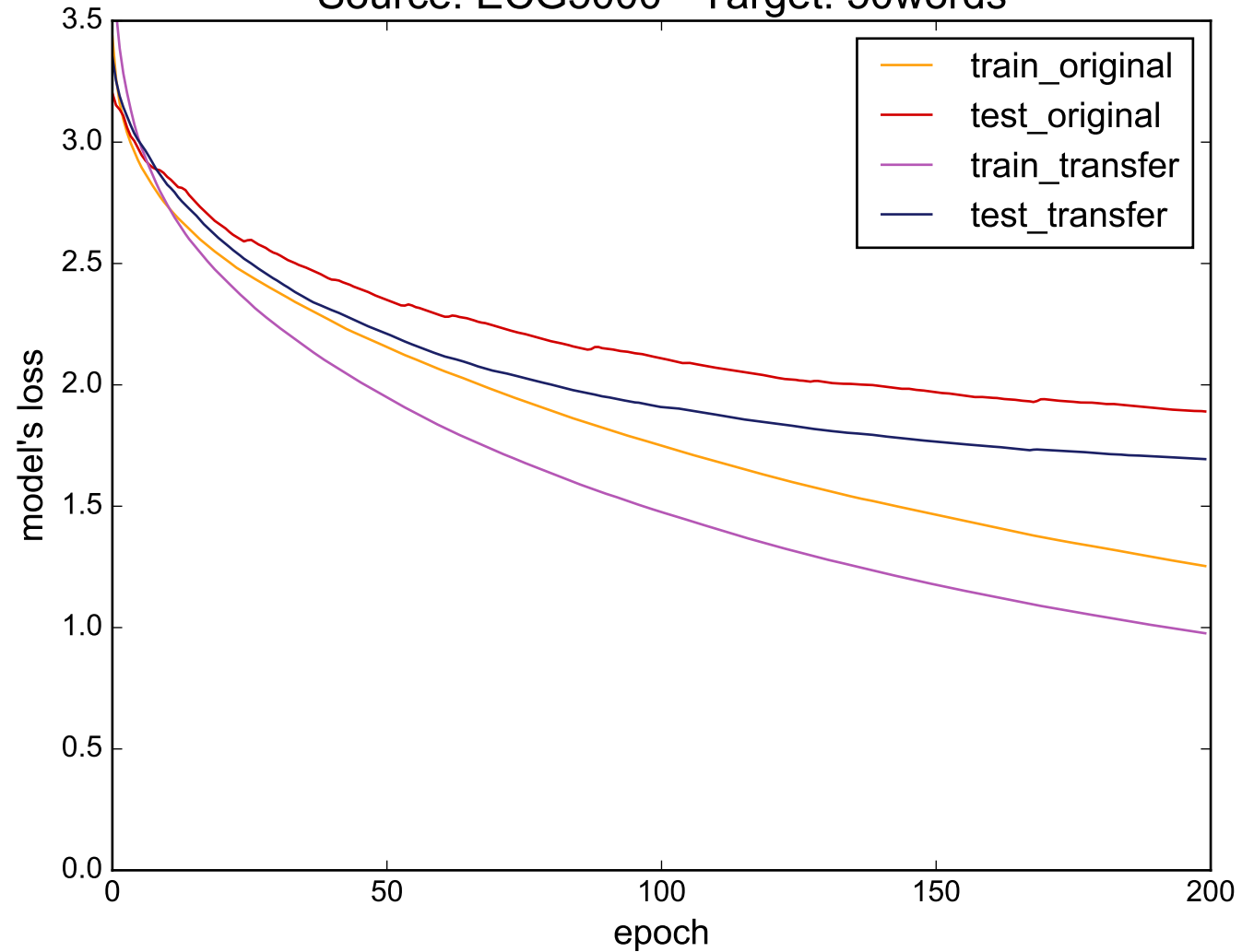
Source: ECG5000 - Target: 50words
