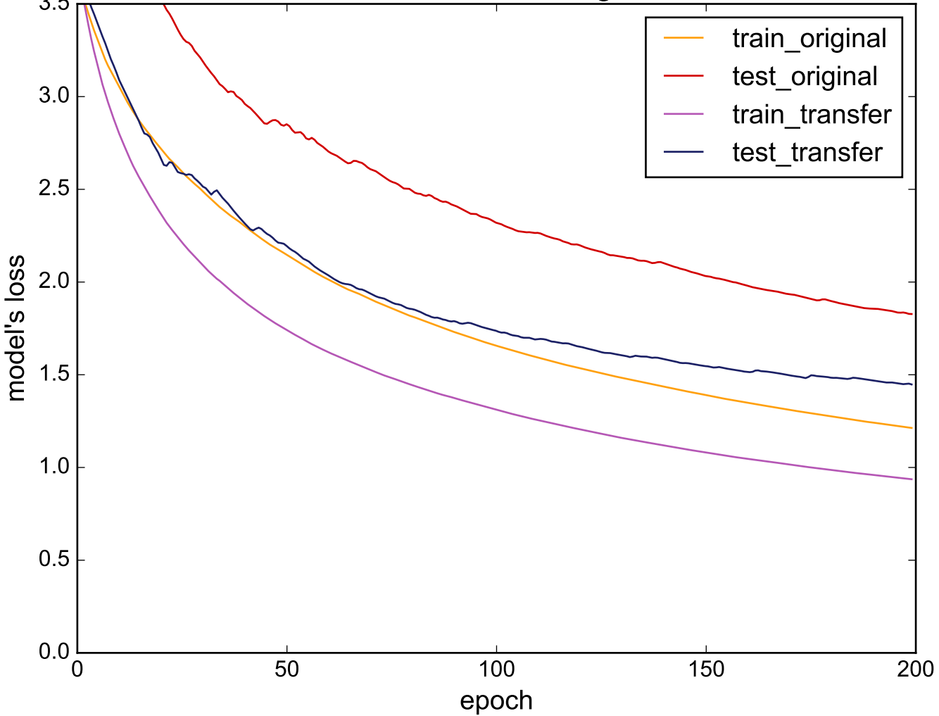
Source: ECG5000 - Target: Adiac
