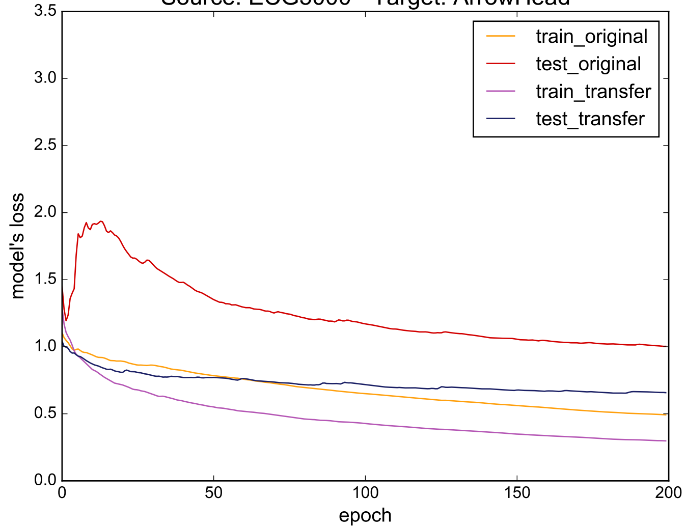
Source: ECG5000 - Target: ArrowHead
