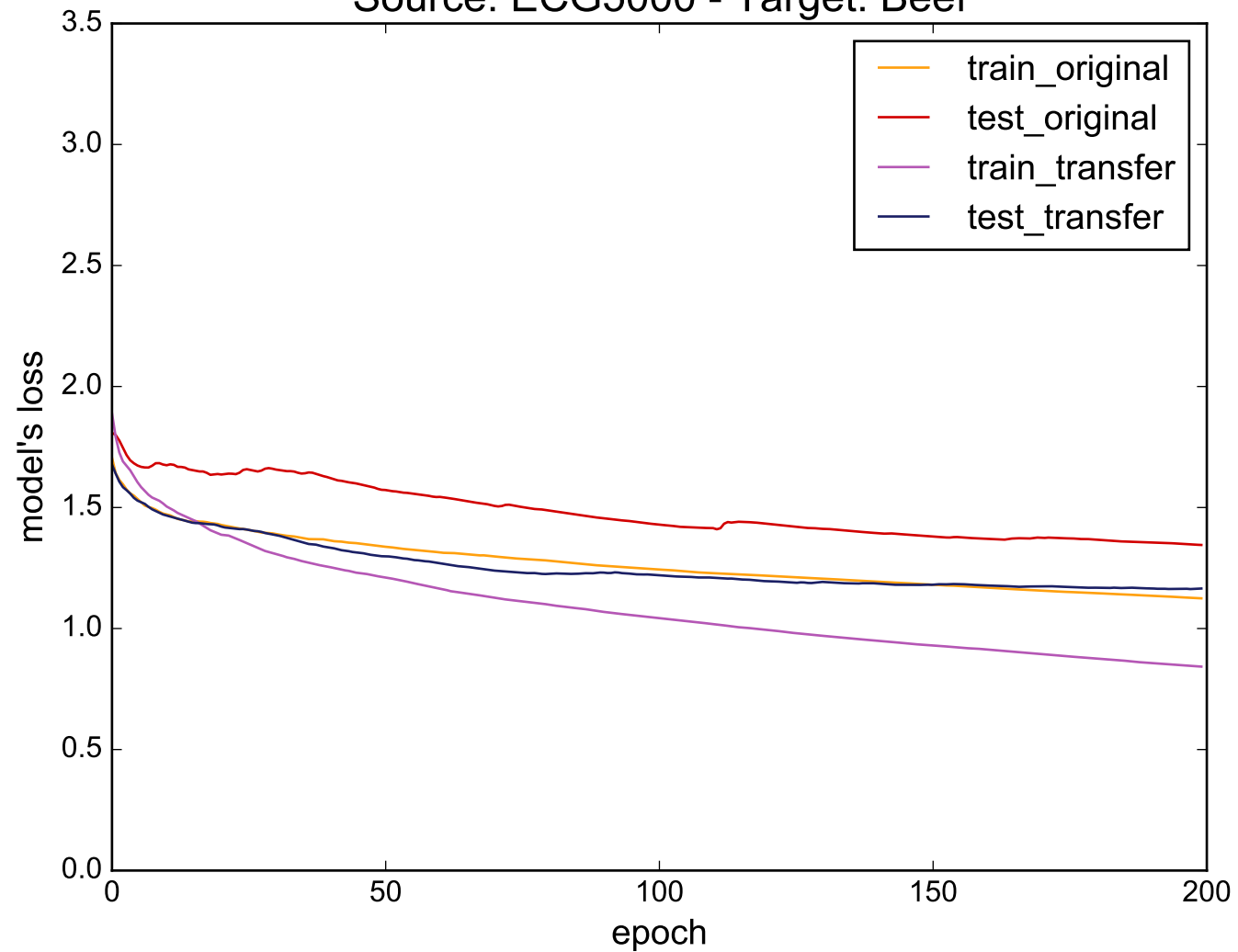
Source: ECG5000 - Target: Beef
