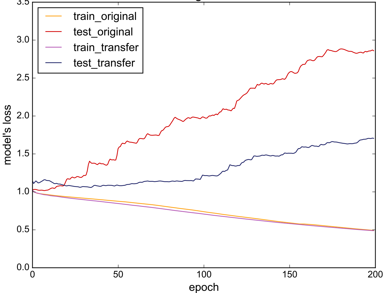
Source: ECG5000 - Target: ChlorineConcentration
