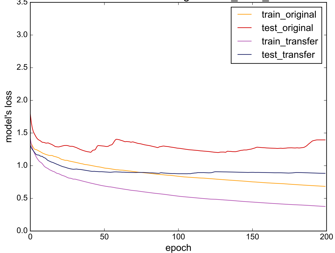
Source: ECG5000 - Target: CinC_ECG_torso
