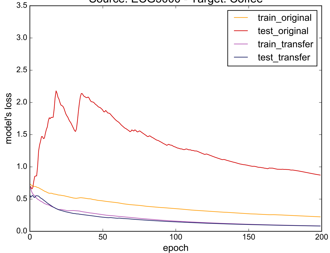
Source: ECG5000 - Target: Coffee
