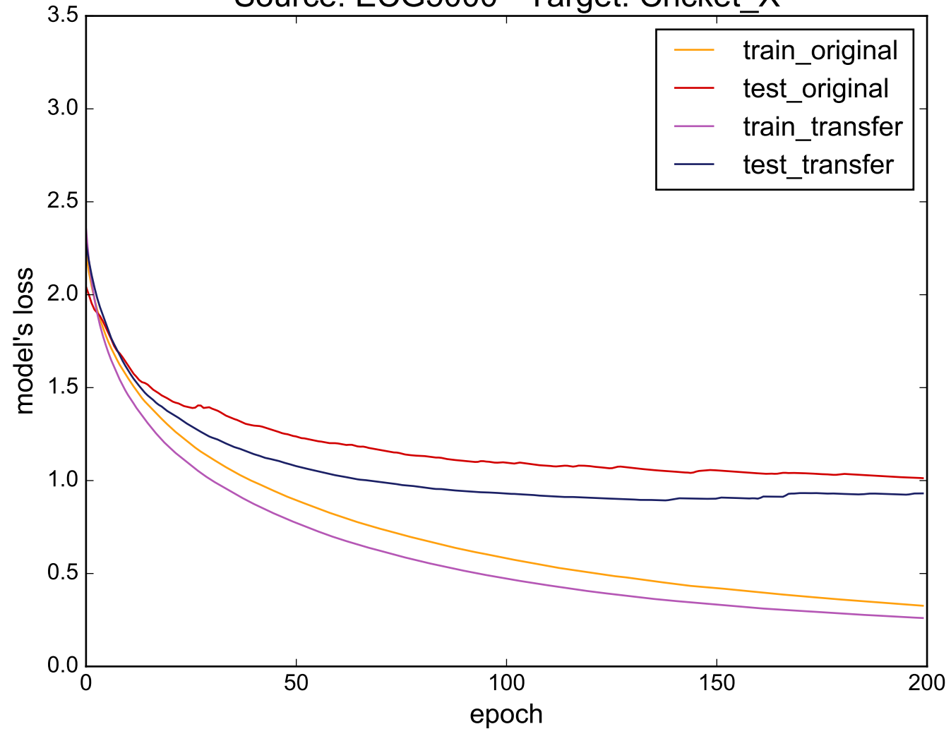
Source: ECG5000 - Target: Cricket_X
