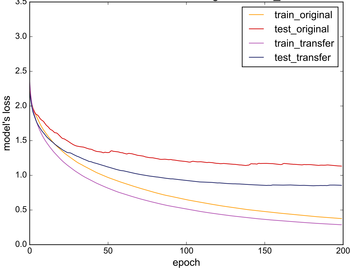
Source: ECG5000 - Target: Cricket_Y
