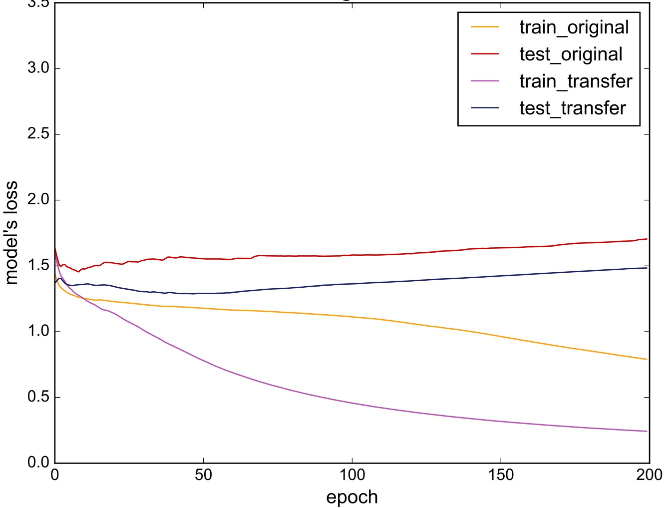
Source: ECG5000 - Target: DiatomSizeReduction
