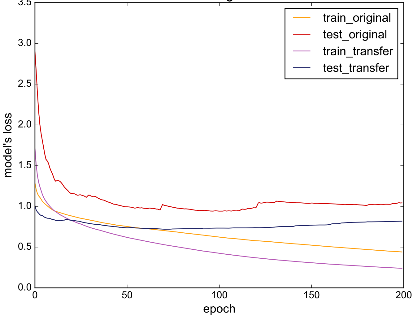
Source: ECG5000 - Target: DistalPhalanxTW
