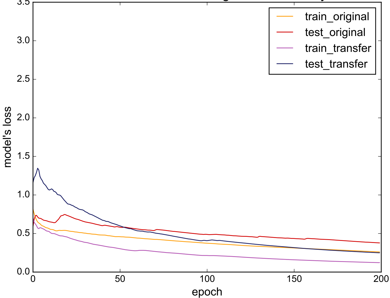
Source: ECG5000 - Target: ECGFiveDays
