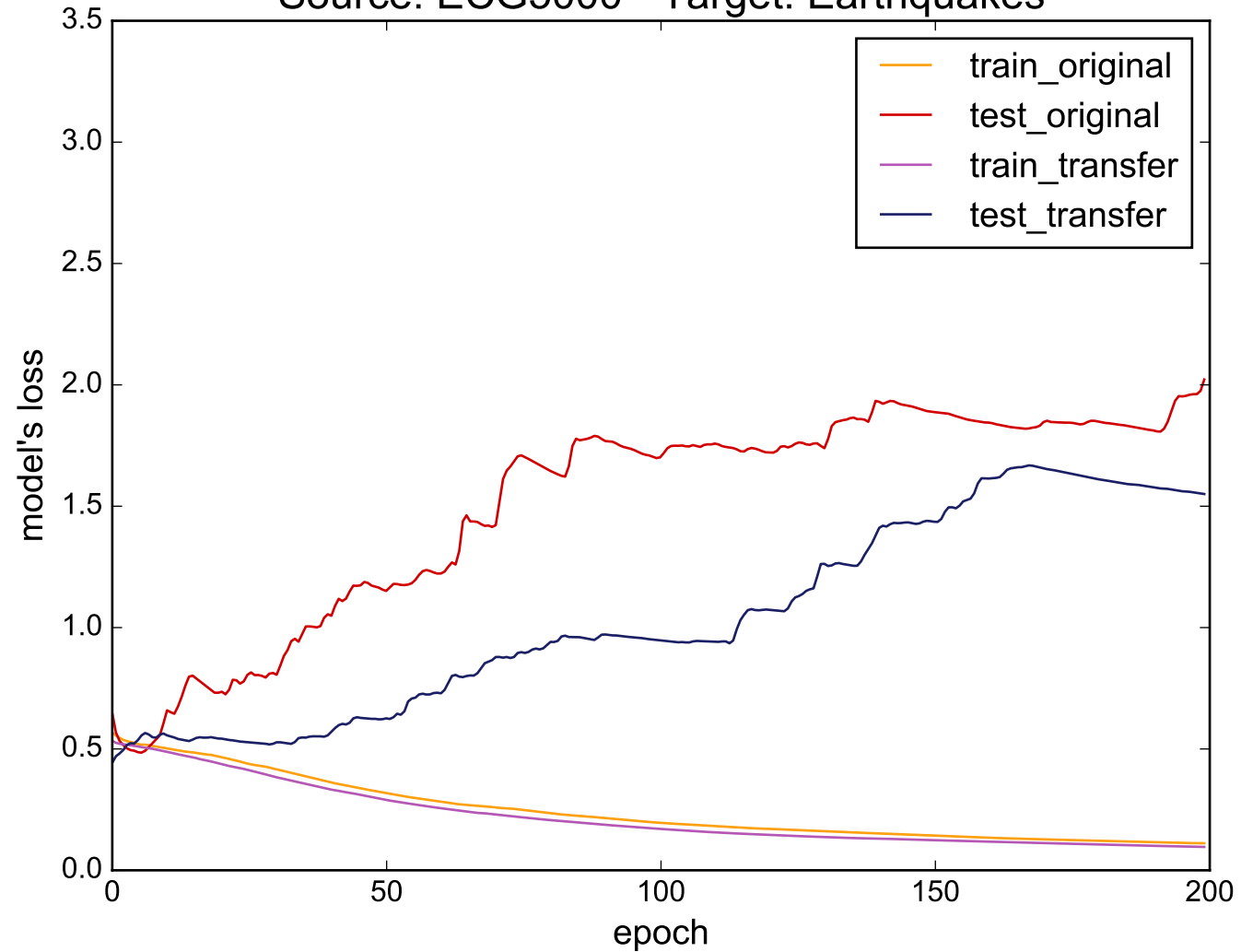
Source: ECG5000 - Target: Earthquakes
