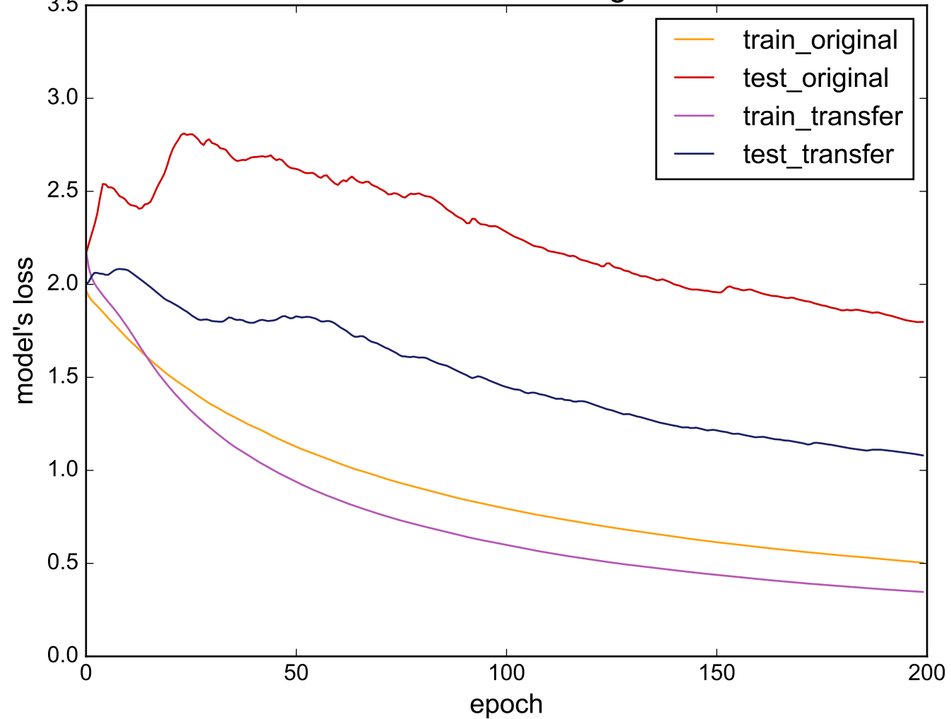
Source: ECG5000 - Target: FISH
