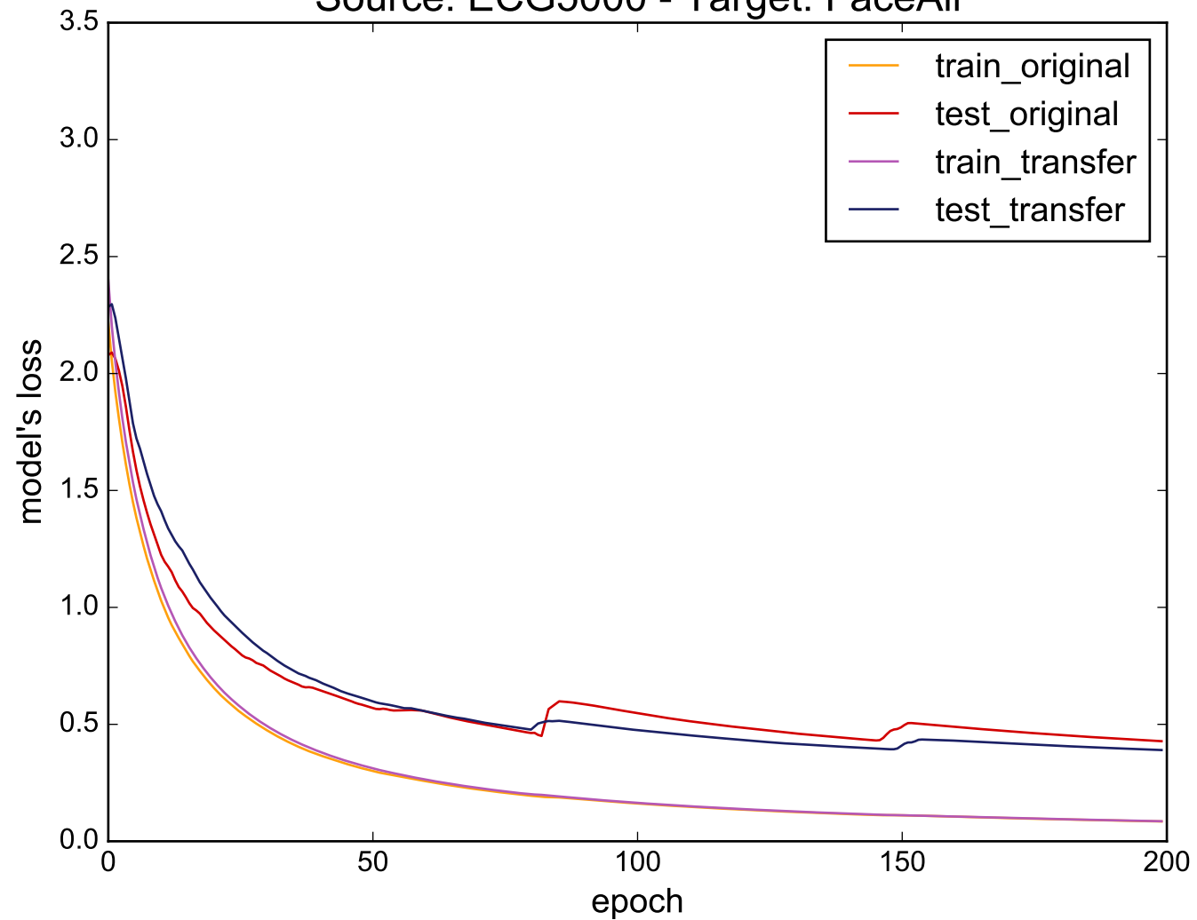
Source: ECG5000 - Target: FaceAll
