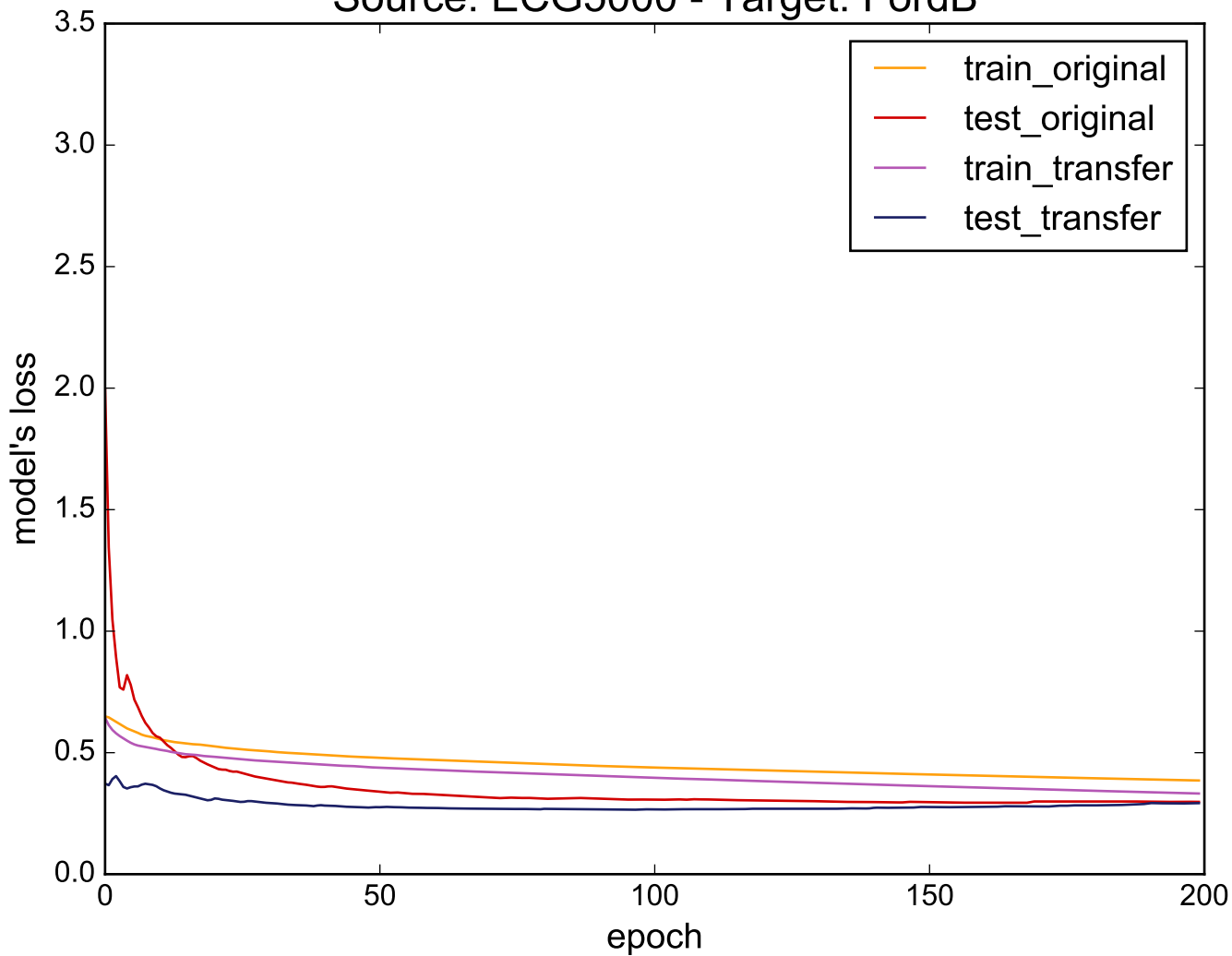
Source: ECG5000 - Target: FordB
