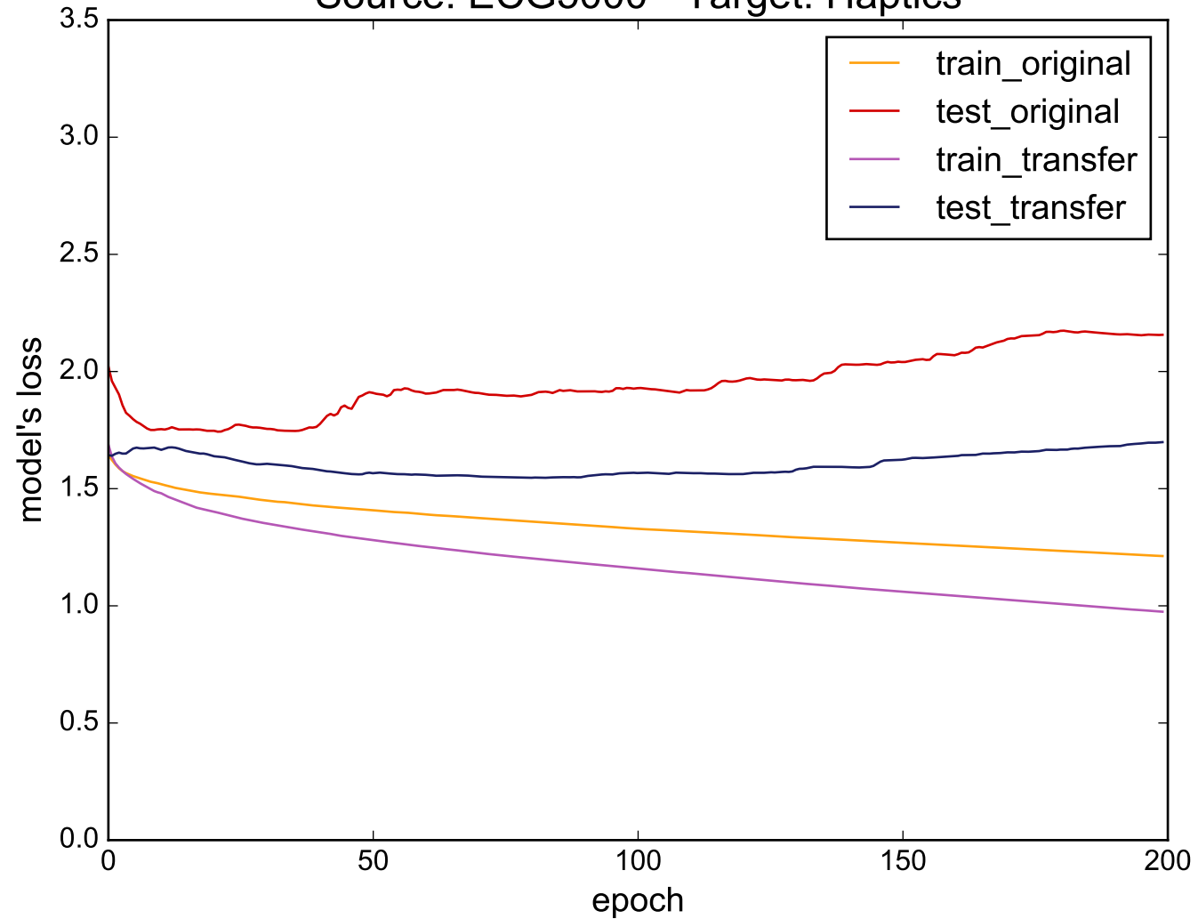
Source: ECG5000 - Target: Haptics
