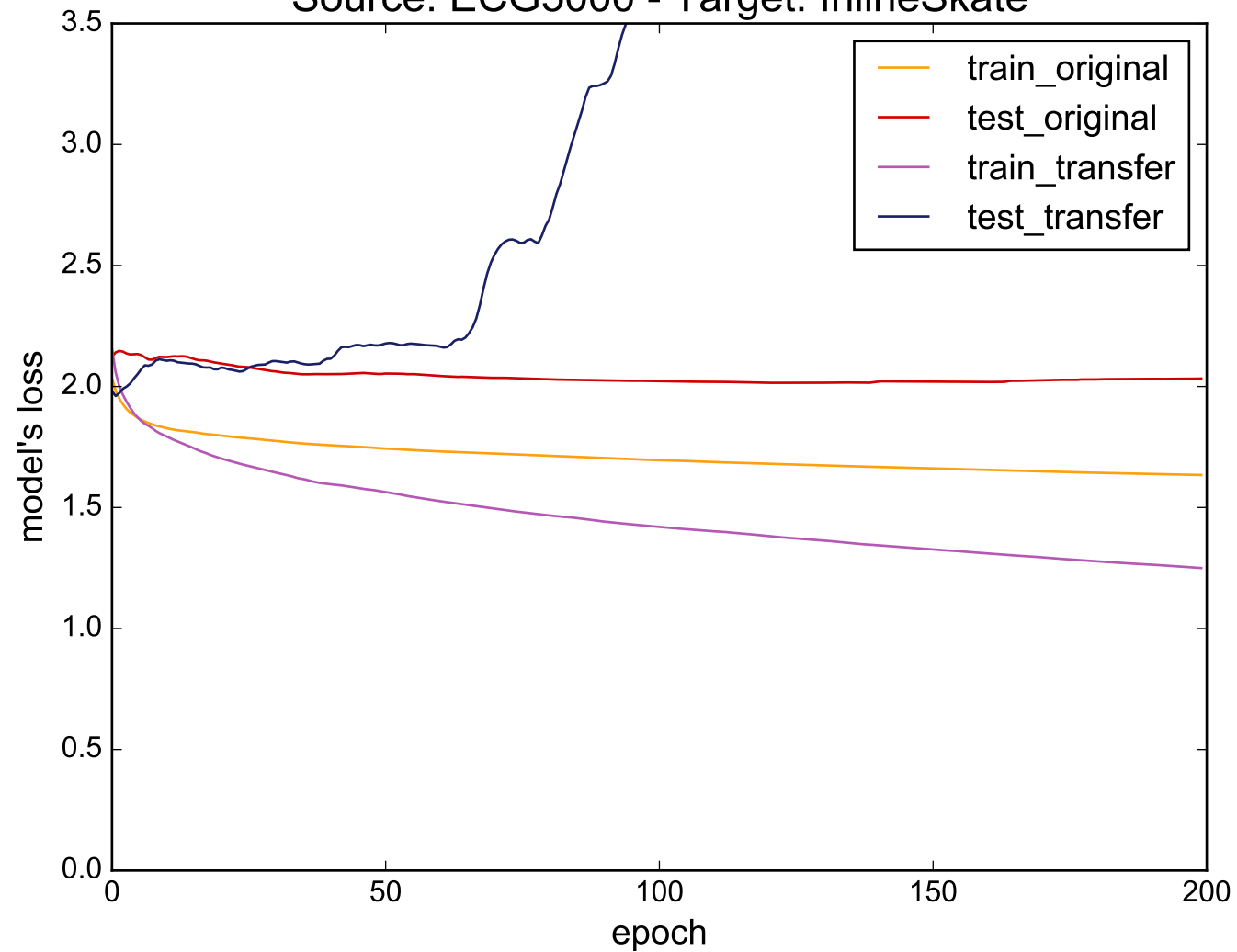
Source: ECG5000 - Target: InlineSkate
