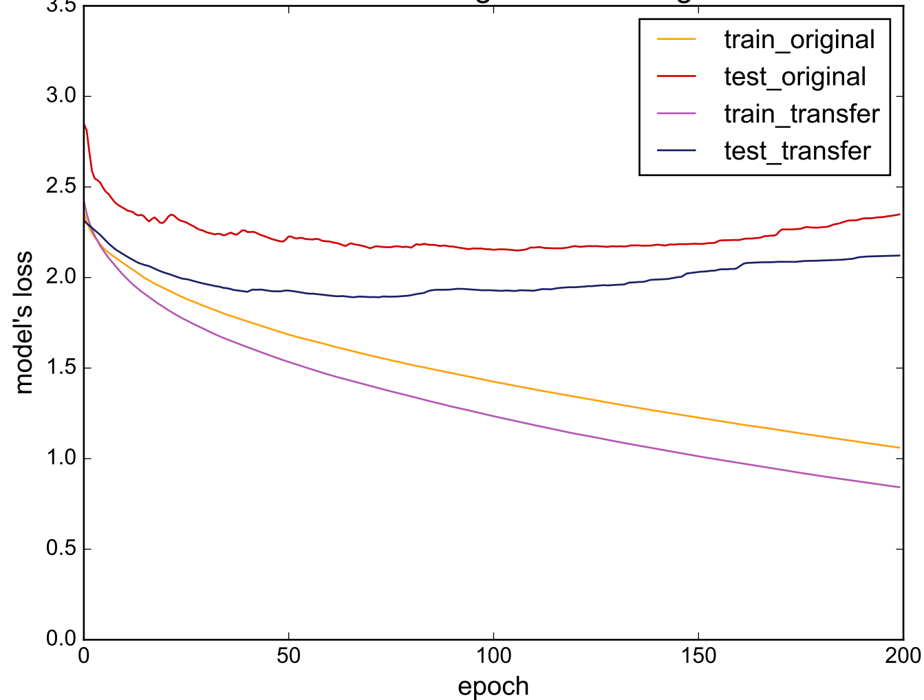
Source: ECG5000 - Target: InsectWingbeatSound
