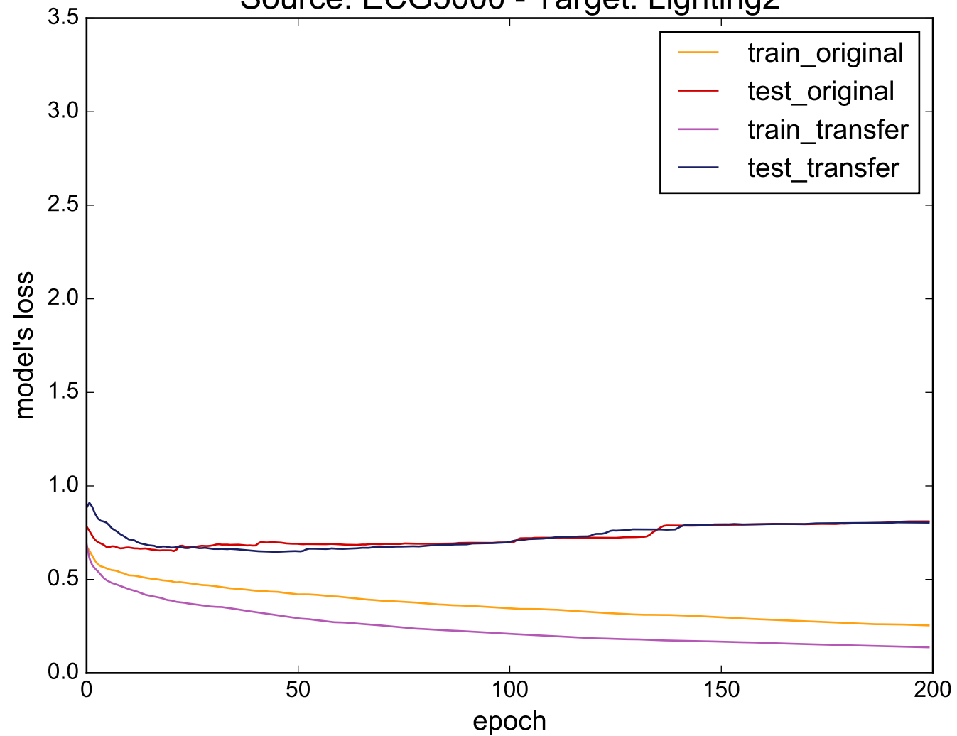
Source: ECG5000 - Target: Lighting2
