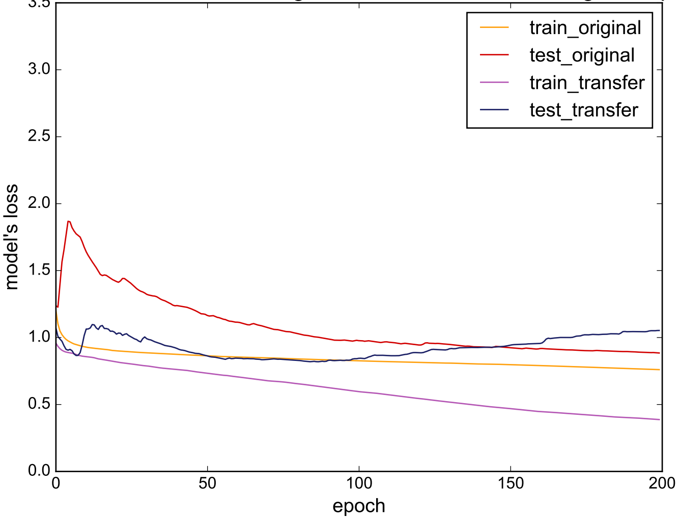
Source: ECG5000 - Target: MiddlePhalanxOutlineAgeGroup
