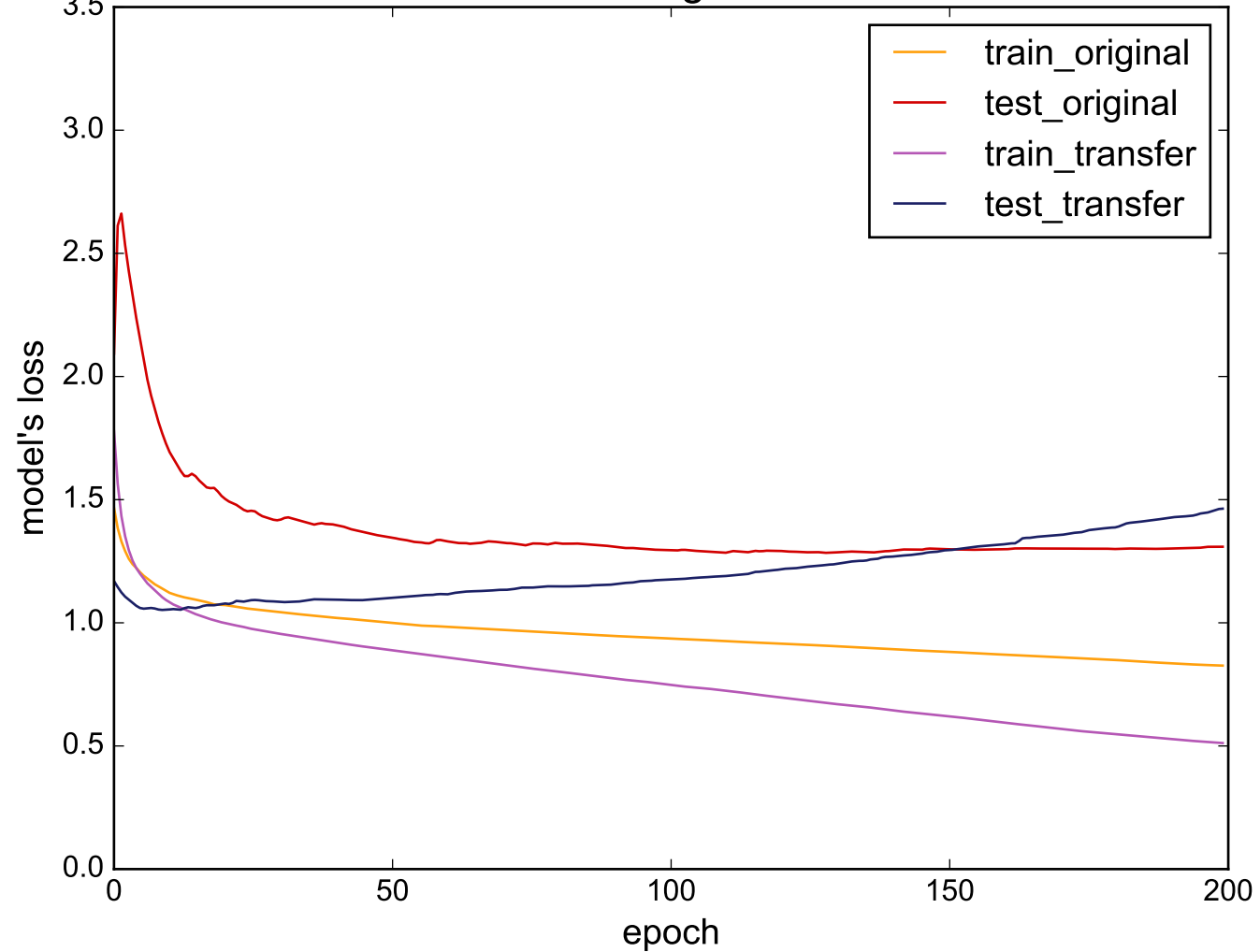
Source: ECG5000 - Target: MiddlePhalanxTW
