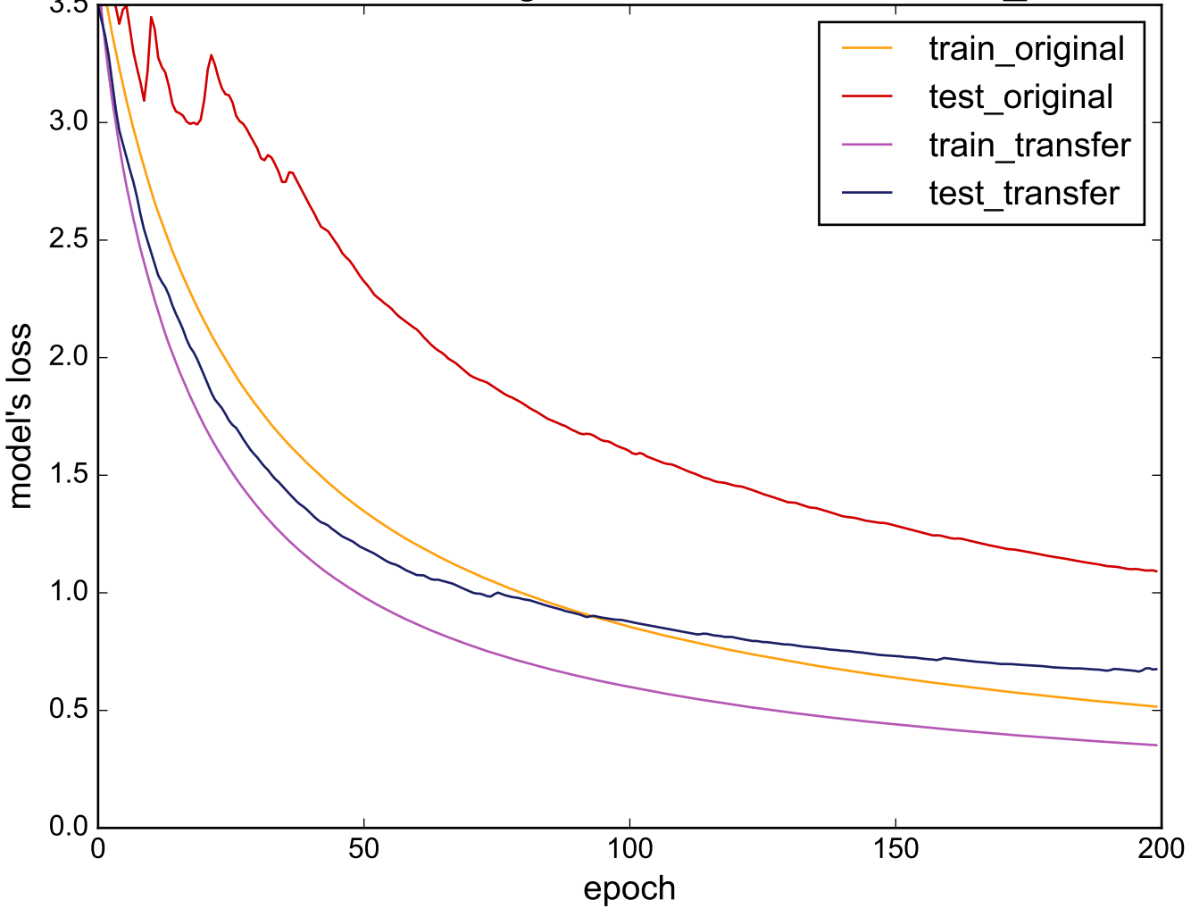
Source: ECG5000 - Target: NonInvasiveFatalECG_Thorax1
