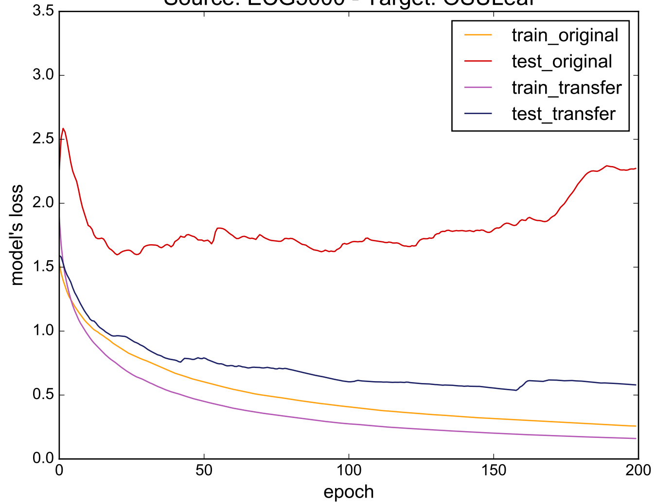
Source: ECG5000 - Target: OSULeaf
