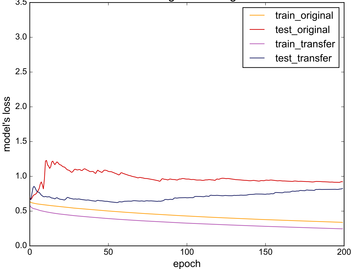
Source: ECG5000 - Target: PhalangesOutlinesCorrect
