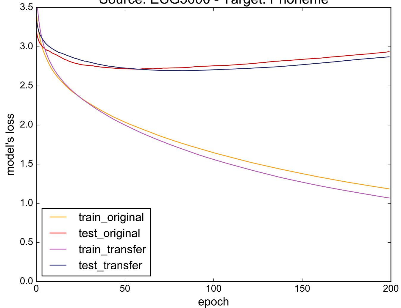
Source: ECG5000 - Target: Phoneme
