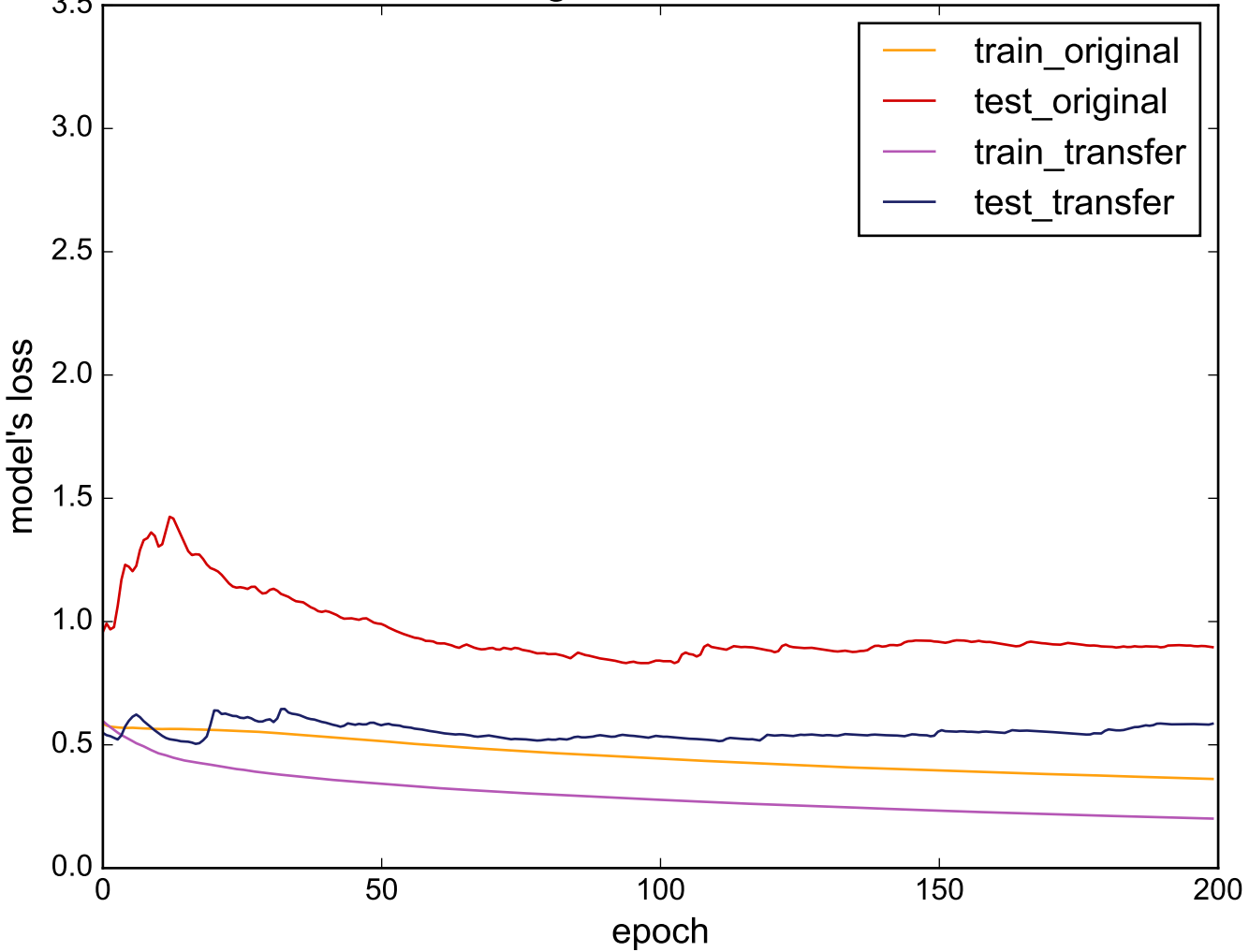
Source: ECG5000 - Target: ProximalPhalanxOutlineCorrect
