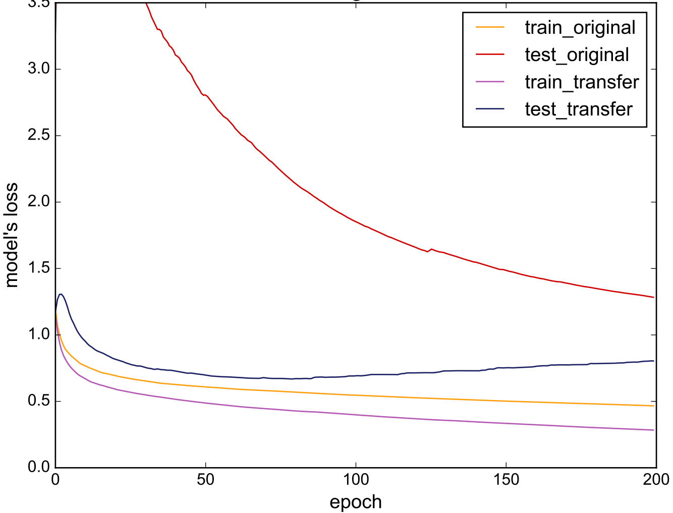
Source: ECG5000 - Target: ProximalPhalanxTW
