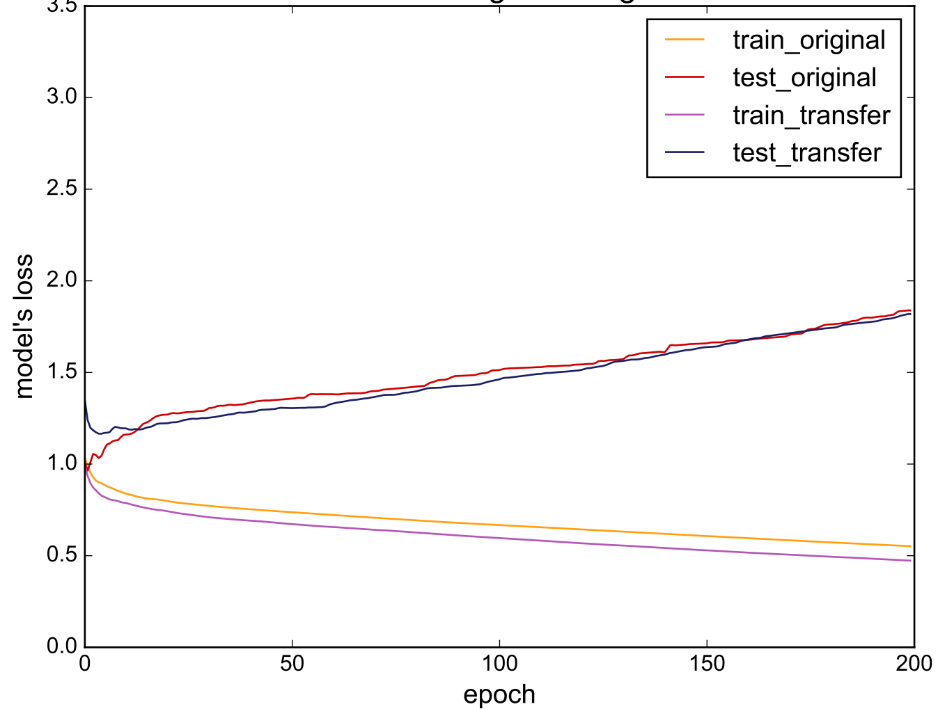
Source: ECG5000 - Target: RefrigerationDevices
