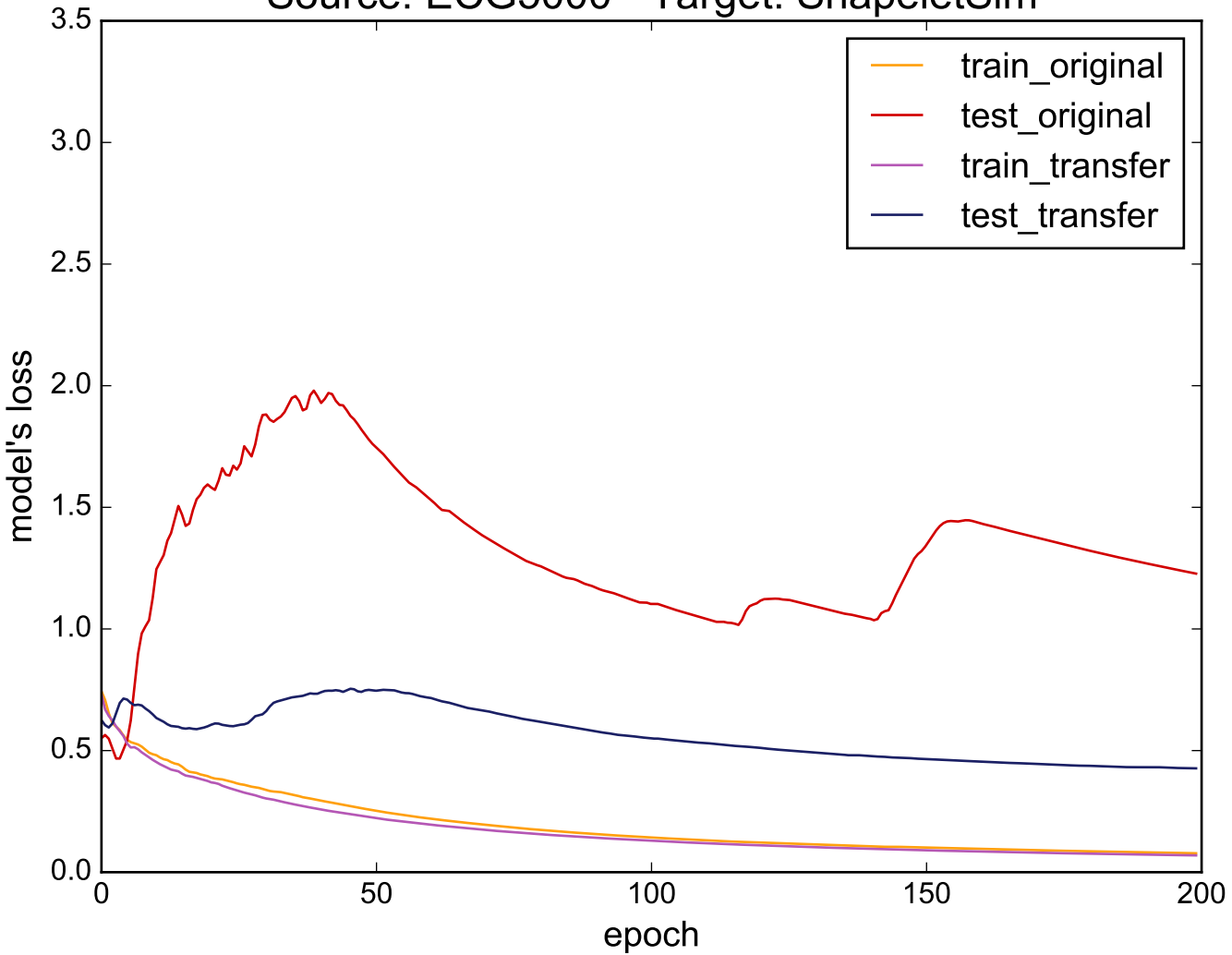
Source: ECG5000 - Target: ShapeletSim
