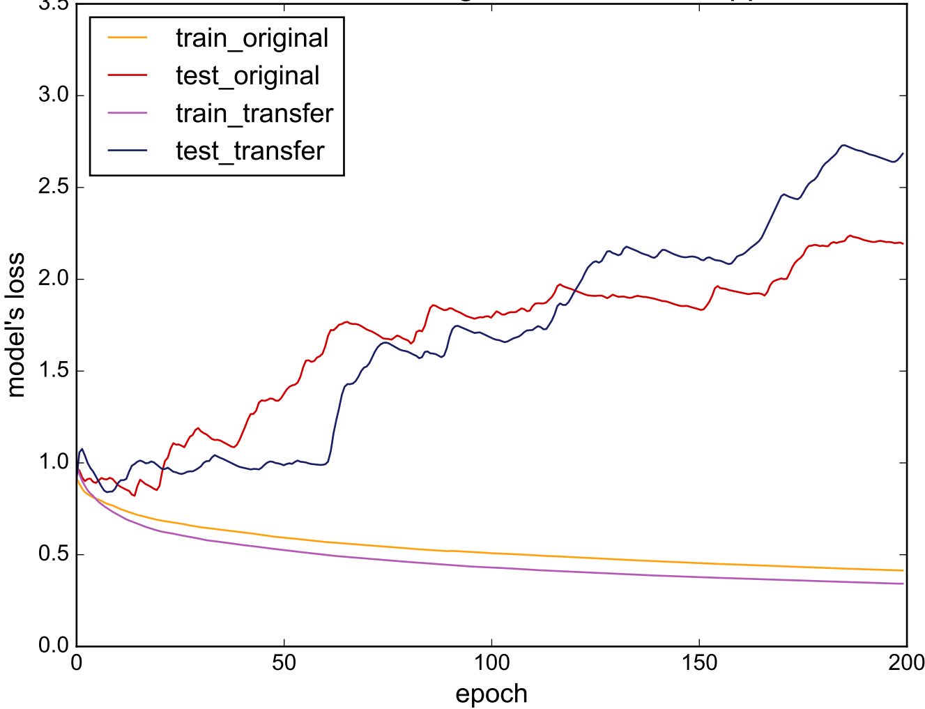
Source: ECG5000 - Target: SmallKitchenAppliances
