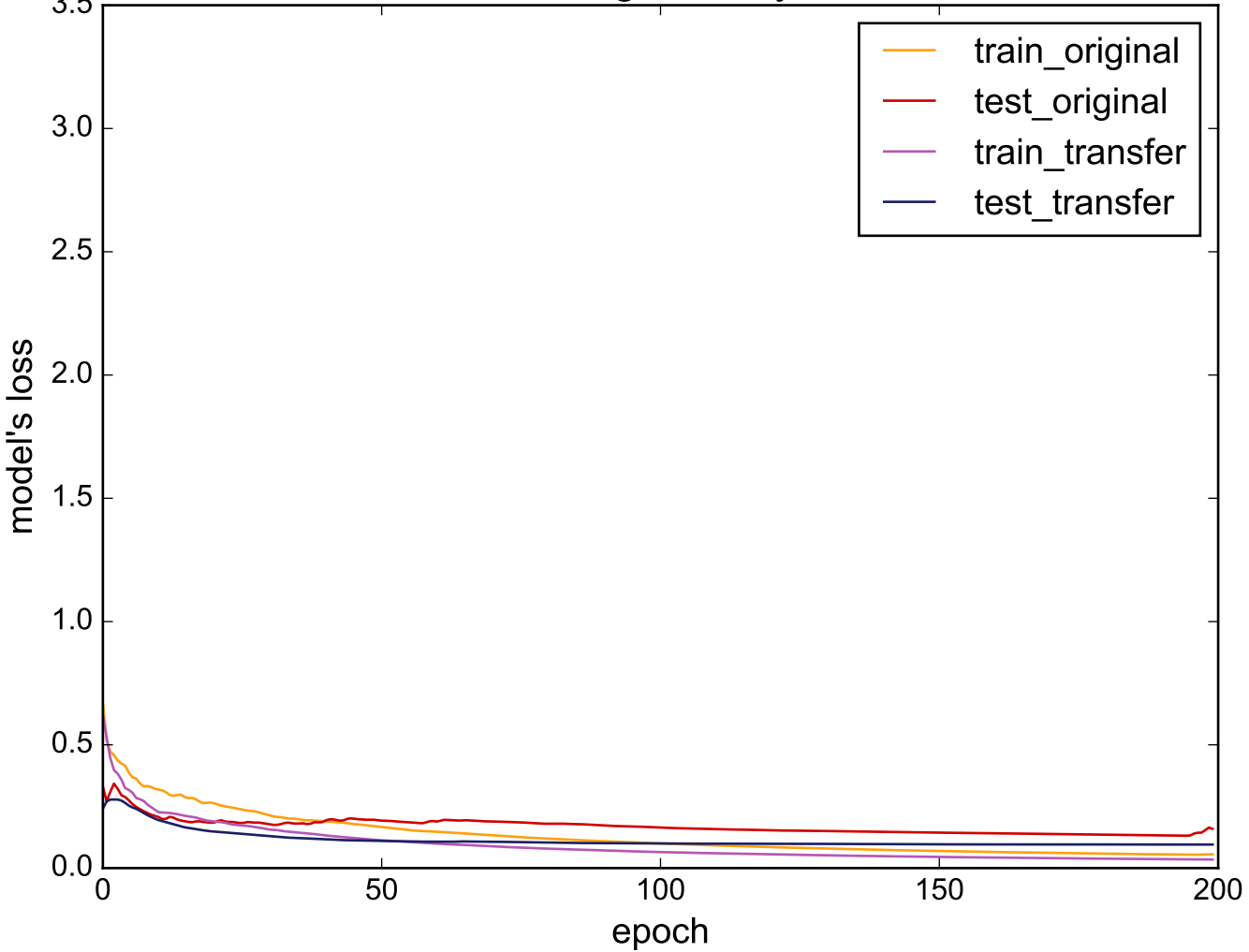
Source: ECG5000 - Target: SonyAIBORobotSurface
