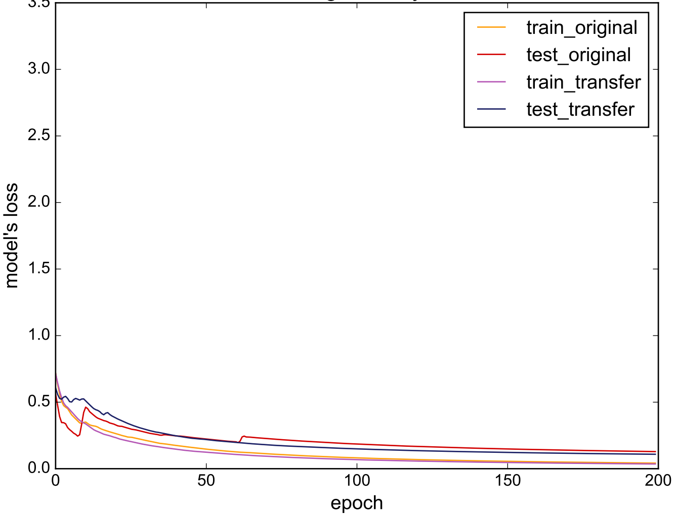
Source: ECG5000 - Target: SonyAIBORobotSurfacell
