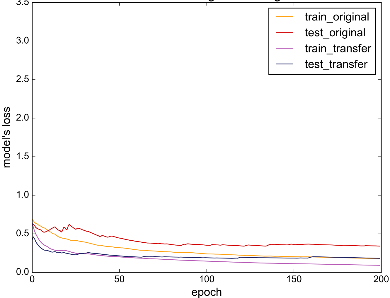
Source: ECG5000 - Target: ToeSegmentation1
