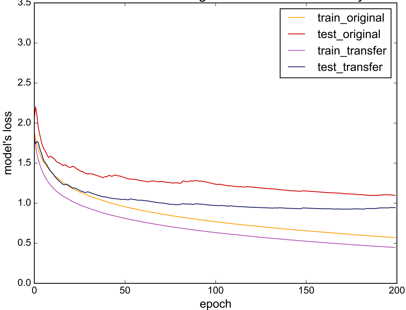
Source: ECG5000 - Target: UWaveGestureLibraryAll
