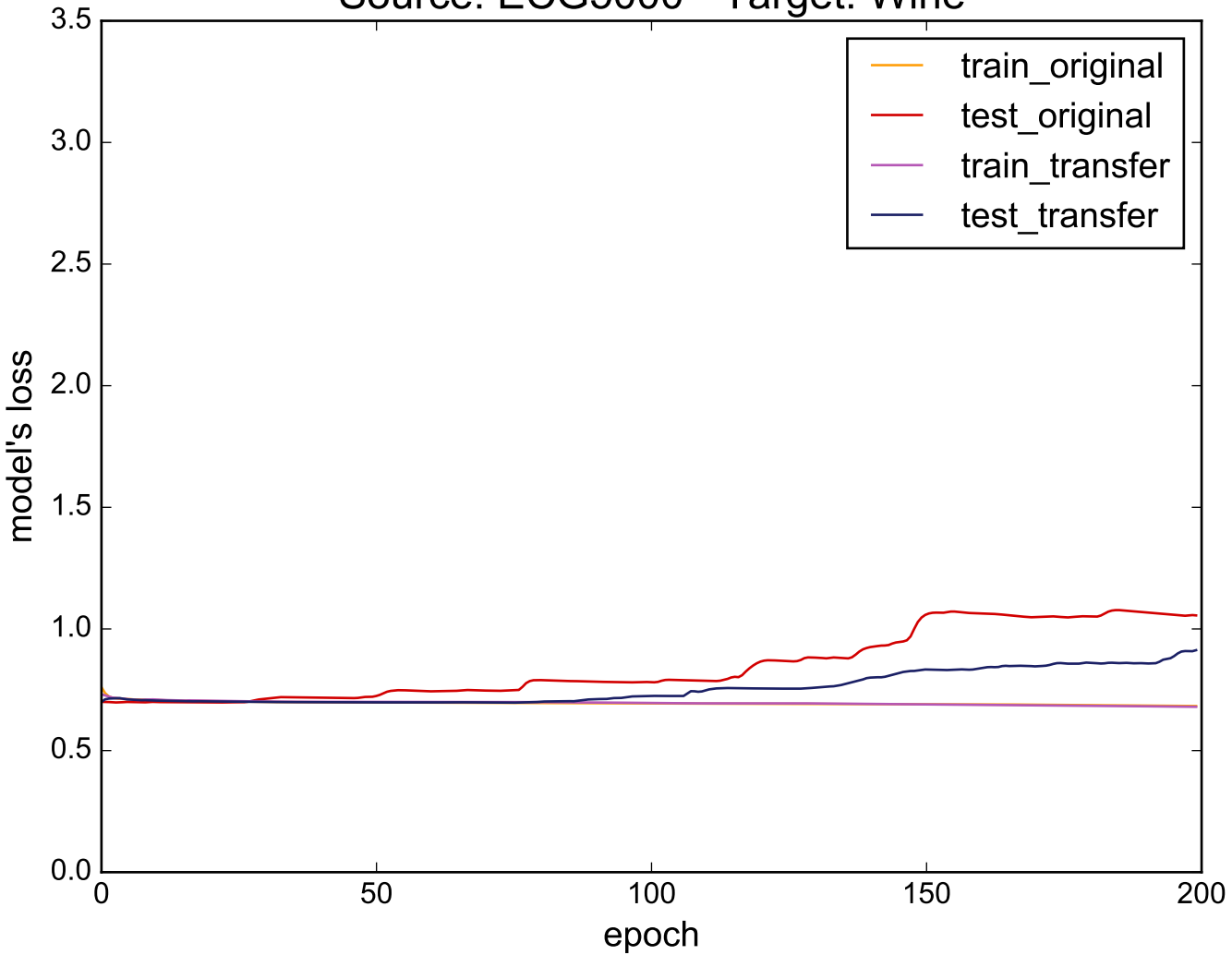
Source: ECG5000 - Target: Wine
