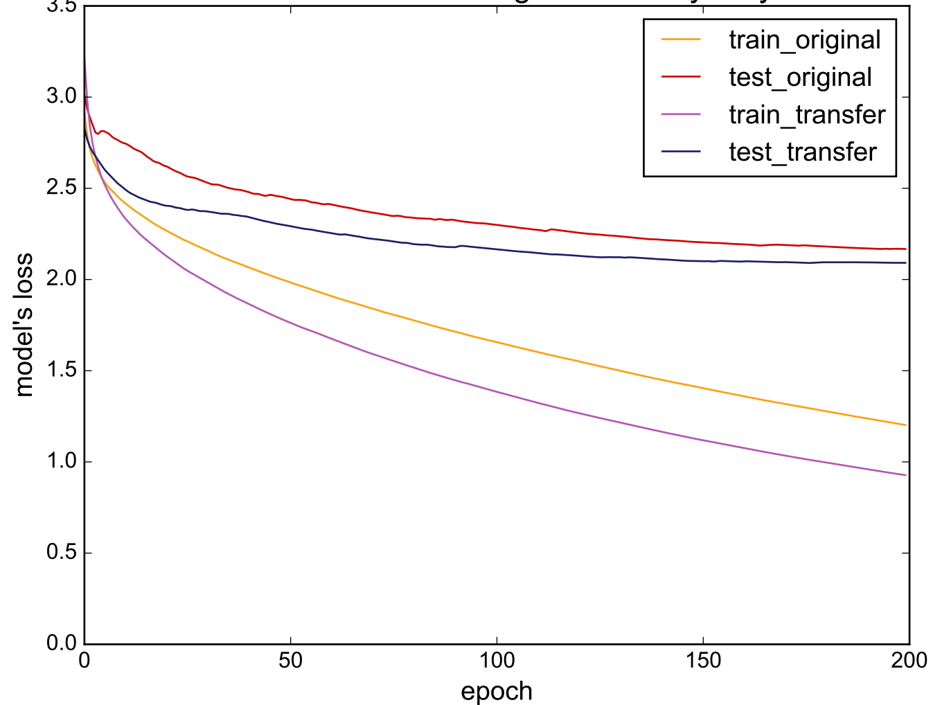
Source: ECG5000 - Target: WordsSynonyms
