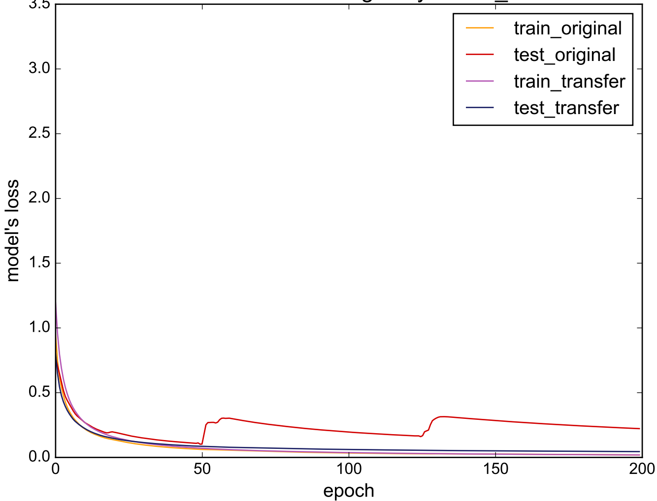
Source: ECG5000 - Target: synthetic_control
