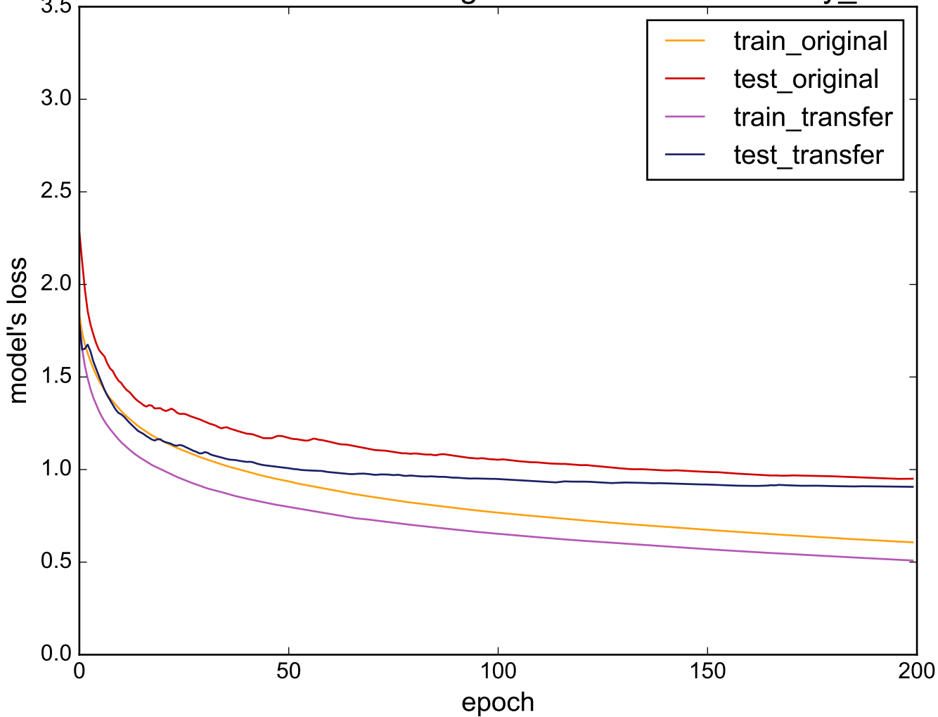
Source: ECG5000 - Target: uWaveGestureLibrary_X
